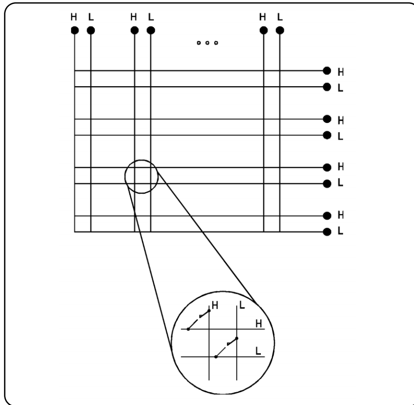
Figure 4. Matrix Configuration
