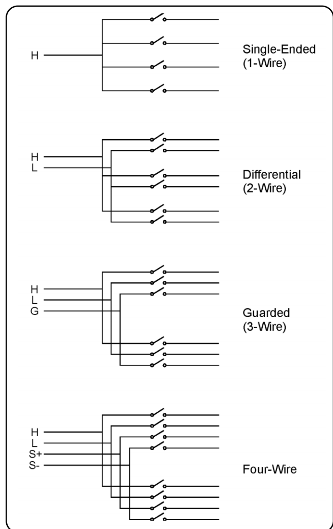
Figure 3. Multiplexer Configurations
